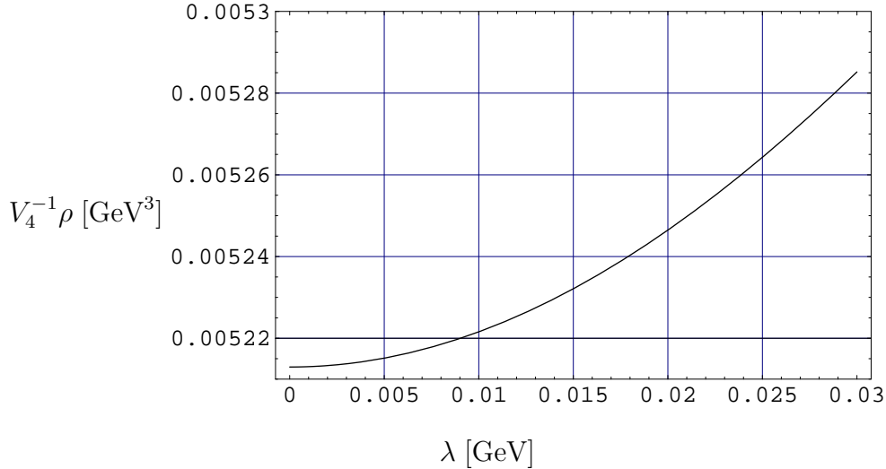
Figure 4: Behaviour of the spectral density at small eigenvalues, which exhibits a quadratic rise due to the absence of a linear contribution in the case N_f=2 .
